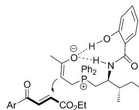
Scheme 2. Proposed transition state model.
